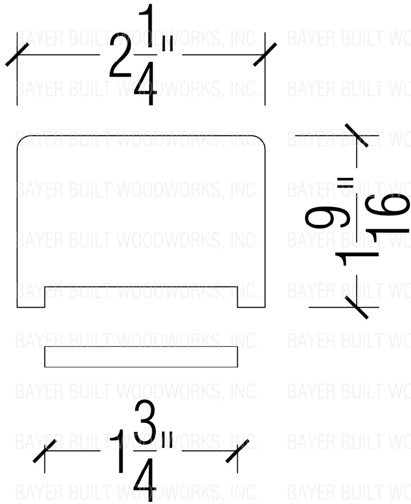
6770P1 HANDRAIL W/ 6007 FILLET
